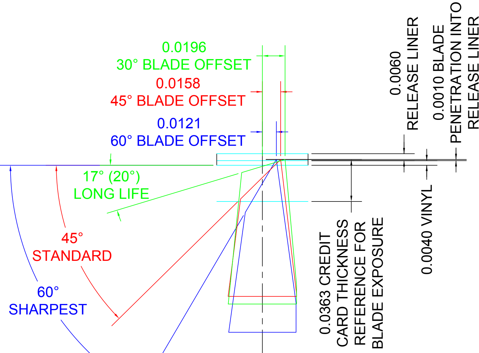
© CutterPros.com and Creation Mechanical and Electrical 2013 ProCut CR Series Blade Angles (Based on actual blade measurements) Dimensions in inches
